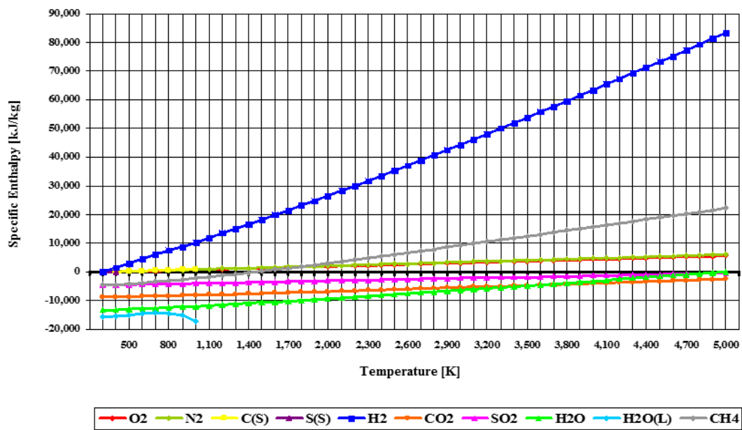
Specific Enthalpy vs Temperature
